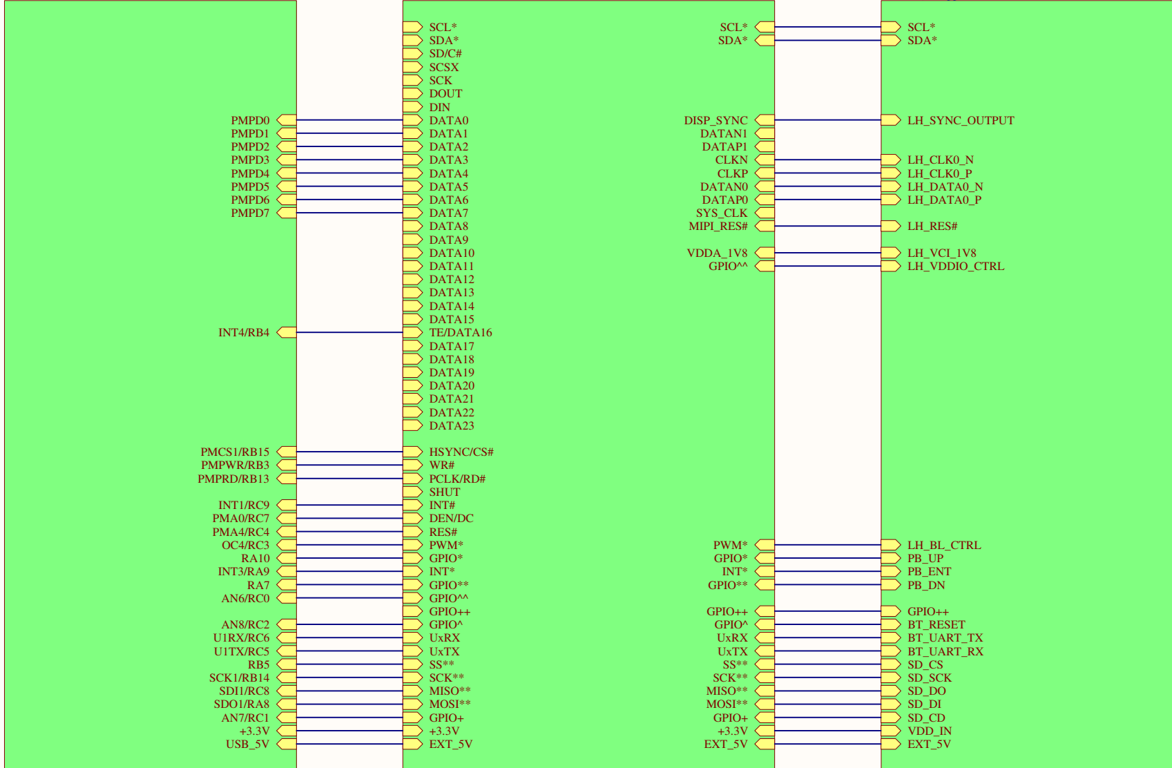
System Diagram of PIC32MX250F128D Host Board + SSD2805 MIPI Bridge + LH154Q01 App Module
